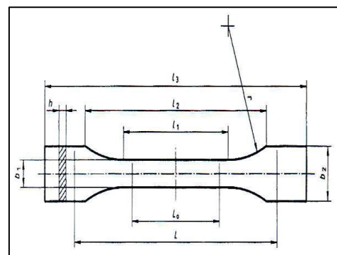
Fig 2: Shape and Dimensions of the Tensile Test Samples
