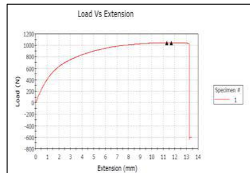
Figure 5: Mechanical Properties at 14 W, Sample 2
