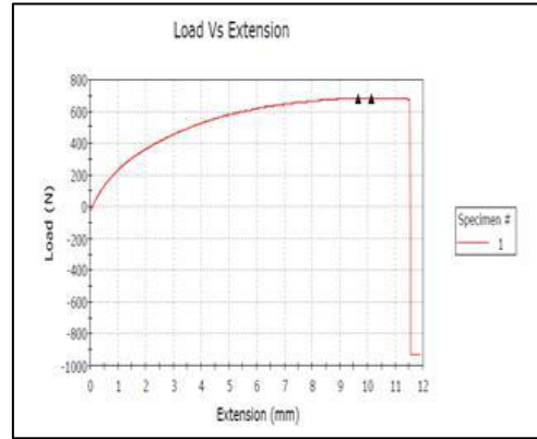
Fig. 4: Mechanical Properties at 14 W, Sample 1
