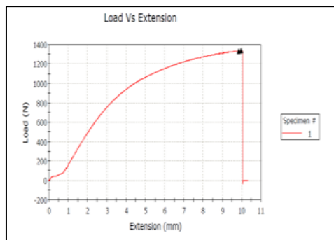
Fig 6: Mechanical Properties at 17 W, Sample 1
