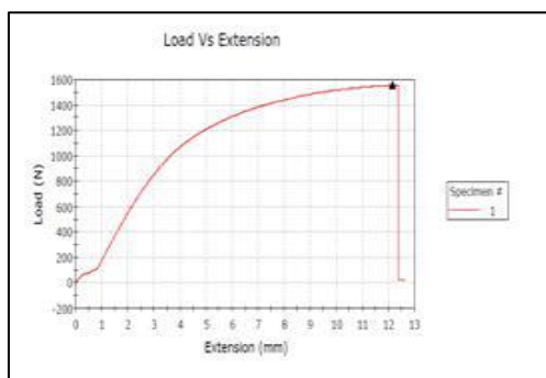
Fig. 7 Mechanical Properties at 17 W, Sample 2
