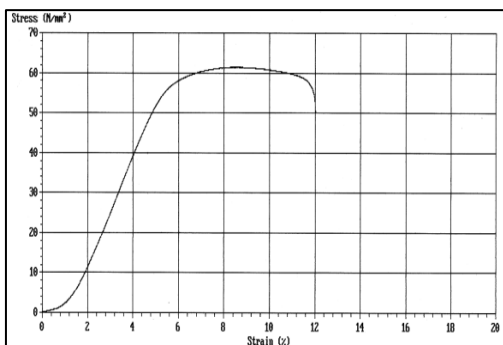
Fig 3: Sample Set – (Laser Power 14 W)
